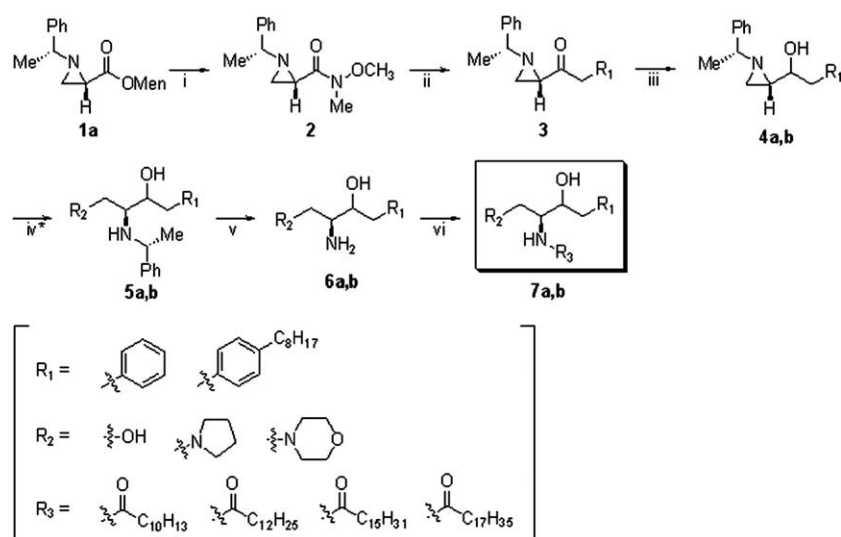
Scheme 1. Reagents and conditions: (i) Weinreb's amine, i -PrMgCl, THF, 0 °C; (ii) benzyl bromide, Mg, THF, 50 °C; (iii) LAH, THF, 0 °C, 85%; (iv)* (a) AcOH, CH 2 Cl 2 , rt, (b) KOH, EtOH, 90% (two steps) or NaI, TMSI, pyrrolidine, MeCN, 90%; (v) Pd(OH) 2 , H 2 , (100 psi), MeOH; (vi) Acyl chloride, NaOH, THF, 76% (two steps).
