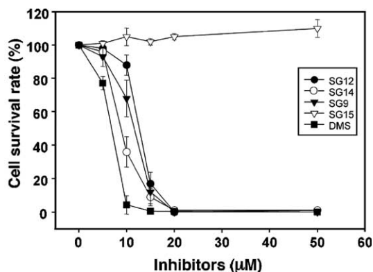
Figure 3. Cytotoxic effects of hSphK inhibitors. The cytotoxic effect was measured using tetrasolium salt. CHO cells ( 5 \times 10^3 cell/100 \mu L) were incubated with the indicated inhibitors at 37 ^{\circ} C for 24 h, then the absorbance of the culture supernatant was measured by spectrophotometry at a wavelength of 450 nm. Data are shown as the percentage of live cells relative to untreated controls from three independent experiments (mean \pm S.D).
