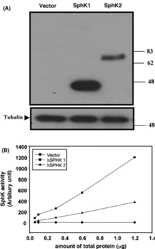
Figure 1. Expression and enzymatic activities of hSphK1 and hSphK2. CHO-K1 cells were transiently transfected with pcDNA3-HA, pcDNA3-HA-hSphK1, or pcDNA3-HA-hSphK2. A. HA-hSphK1 and HA-hSphK2 proteins were separated by SDS-PAGE and analyzed by Western blotting with an anti-HA antibody. An anti-tubulin blot was performed as a loading control. B. Cell lysates were prepared and SphKs activities were measured with 4 μM D-e-sphingosine, 2 μCi[γ- 32 P] ATP, and 0.5 mM cold ATP, at 37 °C for 30 min.
