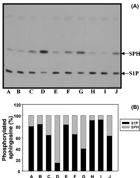
Figure 5. Effect of SphK inhibitors on [ ^3 H] Sphingosine metabolism. Platelet suspensions were pretreated for 5 min with increasing concentrations of SphK inhibitors and then incubated with [ ^3 H] Sphingosine for 15 min. (A) Autoradiography. (B) Quantification of the autoradiography was performed. Data are shown as the percentage of phosphorylated [ ^3 H] sphingosine (S1P) in the total of phosphorylated and unphosphorylated forms of [ ^3 H] Sphingosine. Lane A: negative control, B–D: DMS 5 \mu M, 20 \mu M, 50 \mu M; E–G: SG12 5 \mu M, 20 \mu M, 50 \mu M; H–J: SG14 5 \mu M, 20 \mu M, 50 \mu M.
