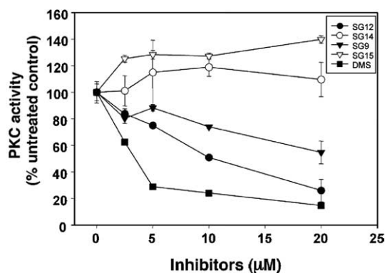
Figure 4. Effect of hSphK2-specific inhibitors on in vitro protein kinase C activity. To monitor the influence of the hSphK2-specific inhibitors on PKC activity, the indicated quantities of inhibitors were supplemented into a PKC assay system containing phosphatidylserine, diacylglycerol, [ \gamma - ^{32} P]ATP and the biotinylated peptide Neurogranin (AAKIQAS*FRGHMARKK). The reaction was initiated by adding 5 ng PKC (an enzyme mixture which consisting of the \alpha , \beta and \gamma isoforms with lesser amounts of the \delta and \zeta isoforms). Data are shown as the percentage of live cells relative to untreated controls from three independent experiments (mean \pm S.D).
