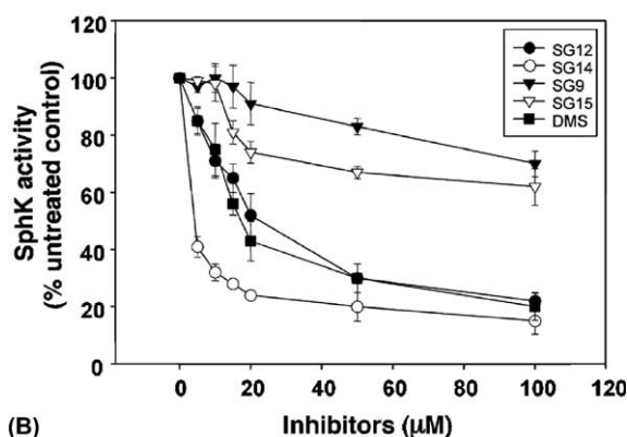
Figure 2. In vitro sphingosine kinase inhibition by sphingoid analogs. (A) Inhibition assays of sphingoid analogs on hSphK1. 1 \mu g protein from lysates of hSphK1-overexpressing CHO-K1 cells were incubated with 4 \mu M D-e-sphingosine, 2 \mu Ci[ \gamma - ^{32} P] ATP, and 0.5 mM cold ATP at 37 ^{\circ} C for 30 min. (B) Inhibition assays of sphingoid analogs on hSphK2. Assays were performed as in A but in the presence of 200 mM KCl and using lysates from the hSphK2-overexpressing CHO-K1 cells. Data are shown as the percentage of SphK activity relative to untreated controls from three independent experiments (mean \pm S.D).
